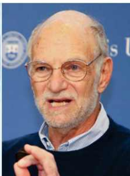
Michael Rosbash
